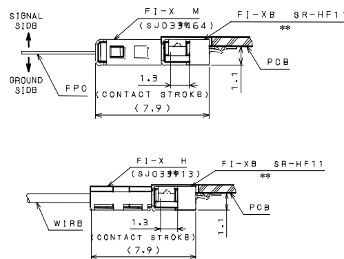
Diagram of connector when mated
