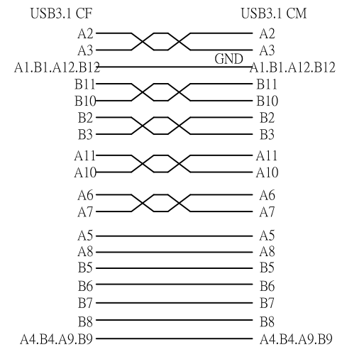
USB3.1CF(Nickel Plated) Black Molding,No:1683 TOL:±0.3
