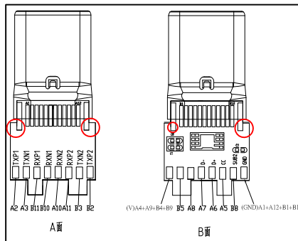
USB 3.1 CM(Nickel Plated) Black Molding,NO:1825 TOL:±0.3
